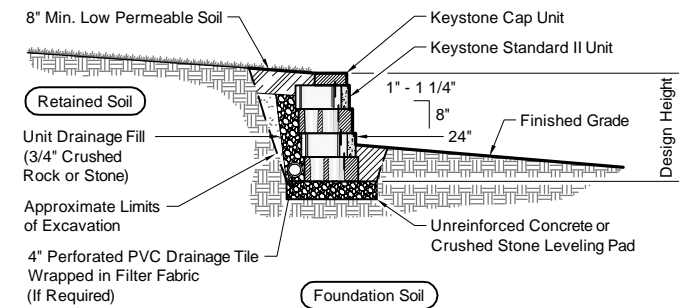
Typical Gravity Wall Section Standard II Unit - 1\"/>
